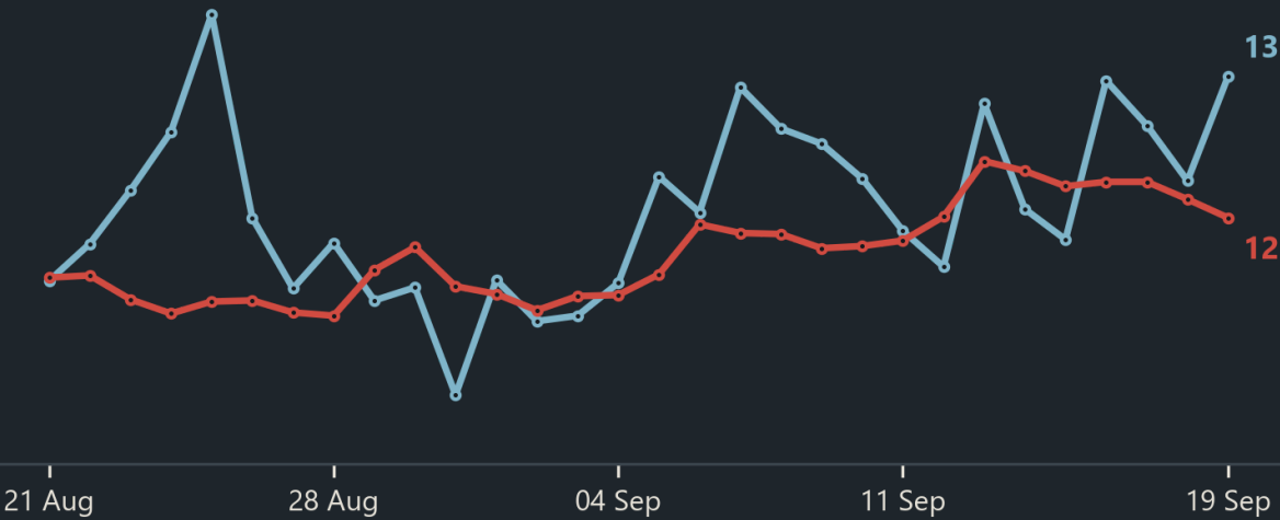
CO, daily level, not a residual (µg/m³)
