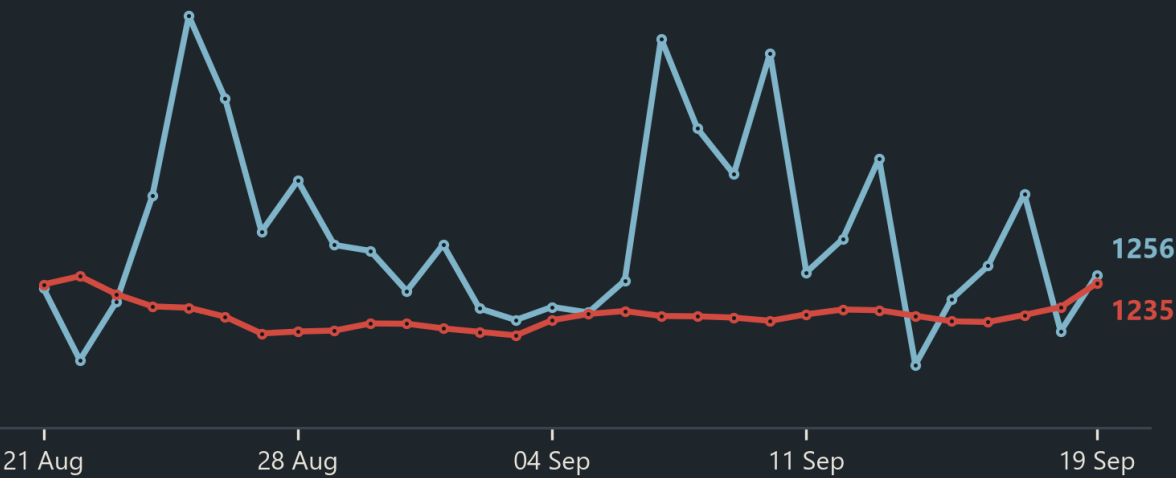
CO, daily level, not a residual (µg/m³)
