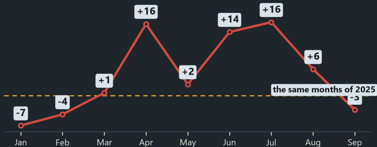
PM10 monthly mean residual, \mu\text{g}/\text{m}^3 against 2025
