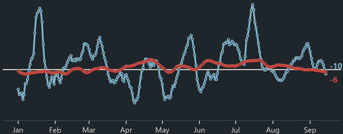
PM10 residual, 2026
